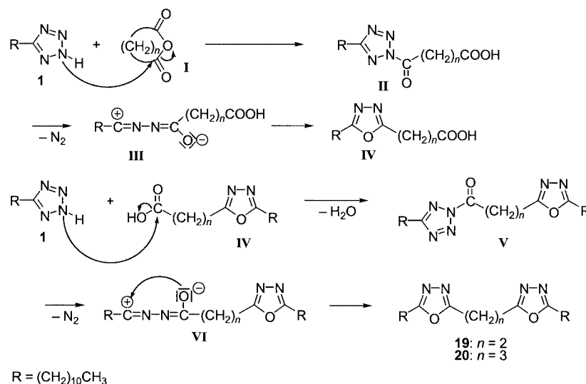
Scheme 3. Reaction pathway to the long-chain bis(oxadiazoles) 19 and 20 by treatment of 5-undecyl-1 H -tetrazole ( 1 ) with succinic and glutaric anhydride, respectively
