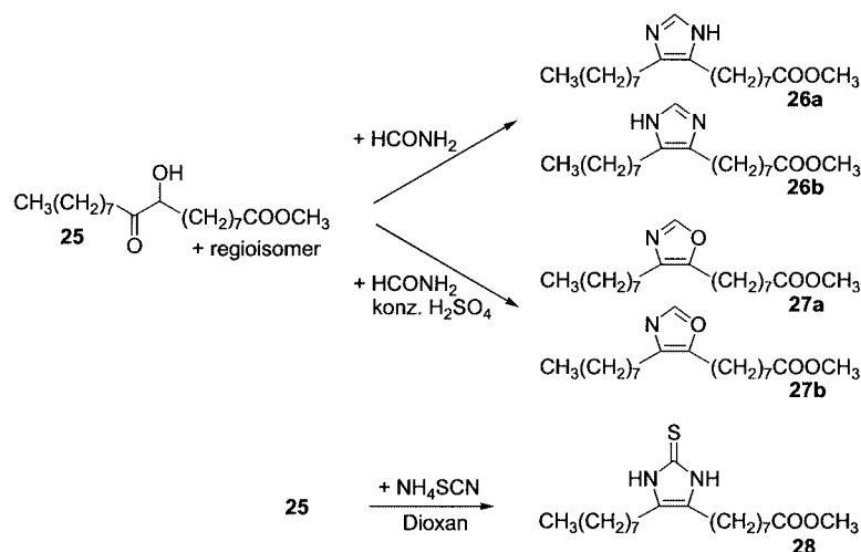
Scheme 6. Reaction of the hydroxy ketone 25 with formamide to give the imidazoles 26 and the oxazoles 27 , and with ammonium thiocyanate to give the imidazolinethione 28
