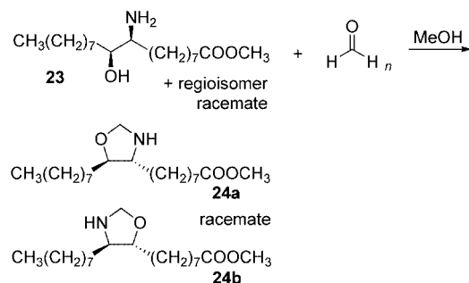
Scheme 5. Condensation of the amino alcohols 23 with paraformaldehyde to give the oxazolidines 24
