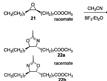
Scheme 4. Formation of the 4,5-dihydrooxazoles 22 from methyl cis -9,10-epoxyoctadecanoate ( 21 ) and acetonitrile in the presence of boron trifluoride–diethyl ether
